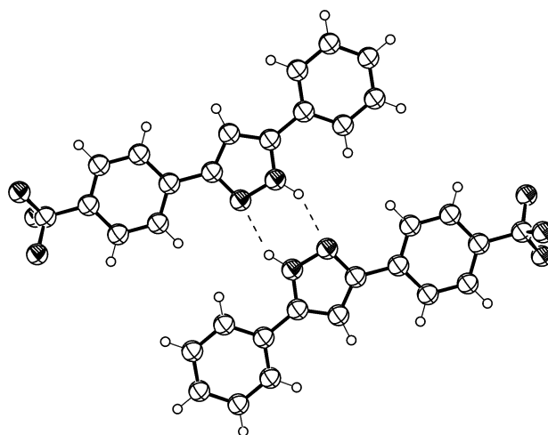
Figure 1. Molecular structure and dimer formation of pyrazole 4e .
