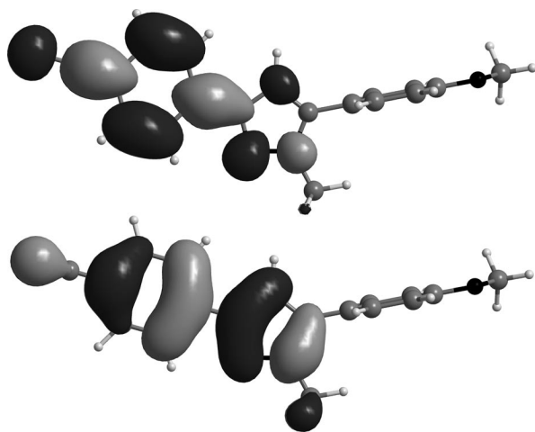
Figure 5. DFT-computed frontier orbitals of pyrazole 4n , LUMO (top) and HOMO (bottom).
