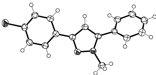
Figure 3. Molecular structure of pyrazole 4l .
