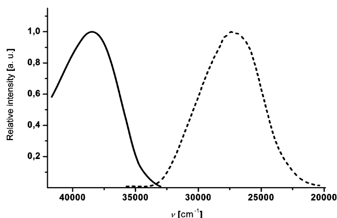
Figure 4. Normalized absorption (solid line) and emission (dotted line) spectra of pyrazole 4k (recorded in CH 2 Cl 2 , 293 K).
