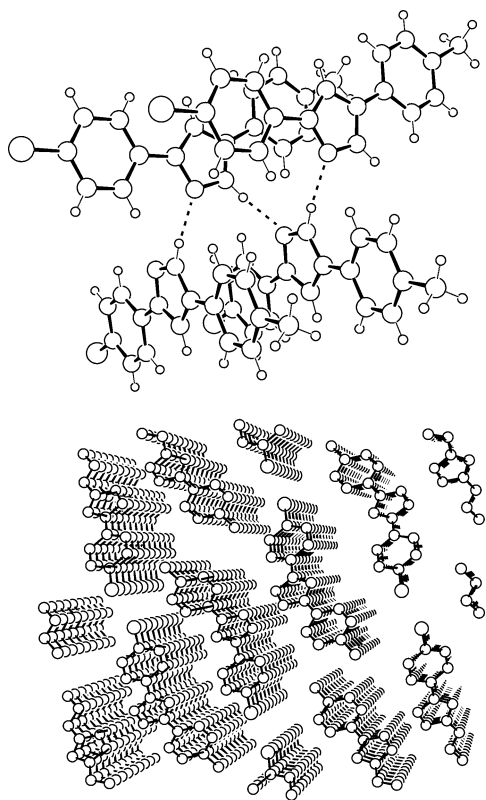
Figure 2. Bridging by hydrogen bonding and \pi -stacking in single crystals of 4c .
