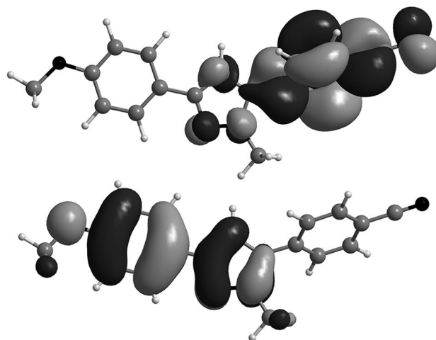
Figure 6. DFT-computed frontier orbitals of pyrazole 4o , LUMO (top) and HOMO (bottom).
