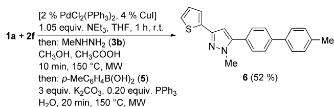
Scheme 3. One-pot four-component synthesis of pyrazole 6 .
