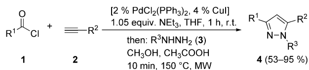
Scheme 2. One-pot three-component synthesis of pyrazoles 4 .
