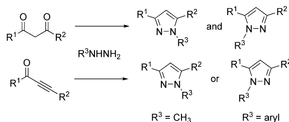
Scheme 1. Variable regioselectivity in pyrazole formation depending on 1,3-diketones and alkynones as C_3 building blocks.
